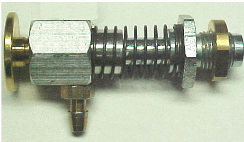
T Style Vacuum Stem : 12 mm Stroke
