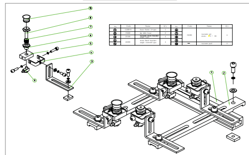
ASSEMBLY Dwg.
