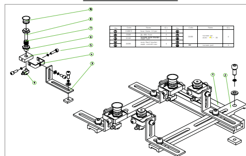
ASSEMBLY Dwg.
