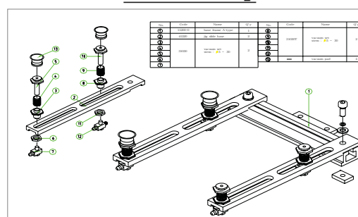
ASSEMBLY Dwg.
