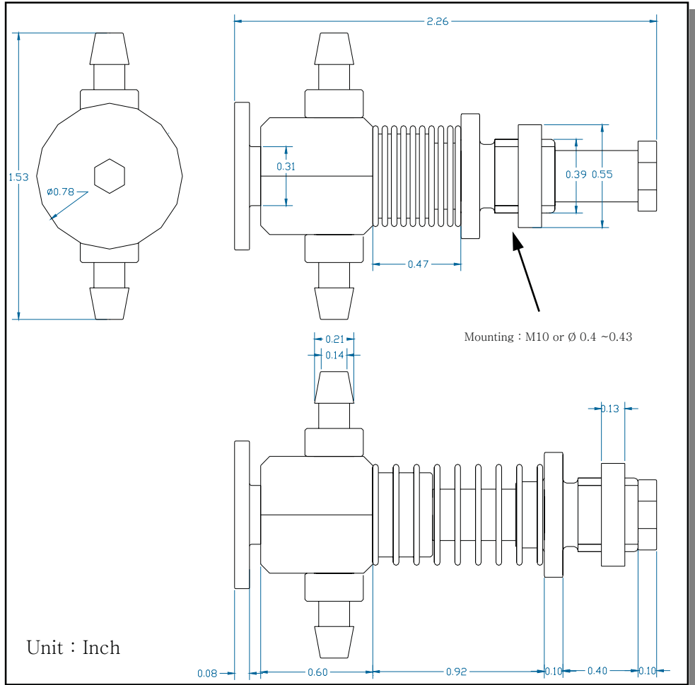
T Style Vacuum Stem : 12 mm Stroke
