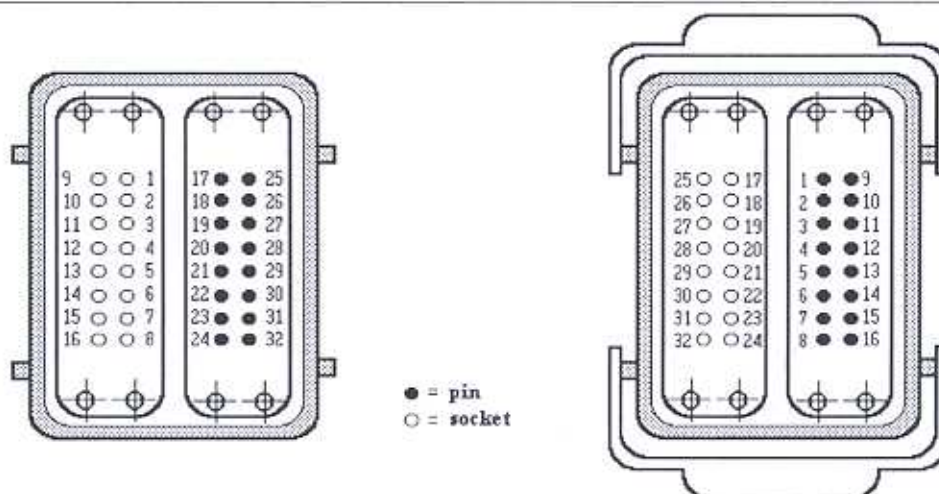
Figure 1: Plug on the handling device
