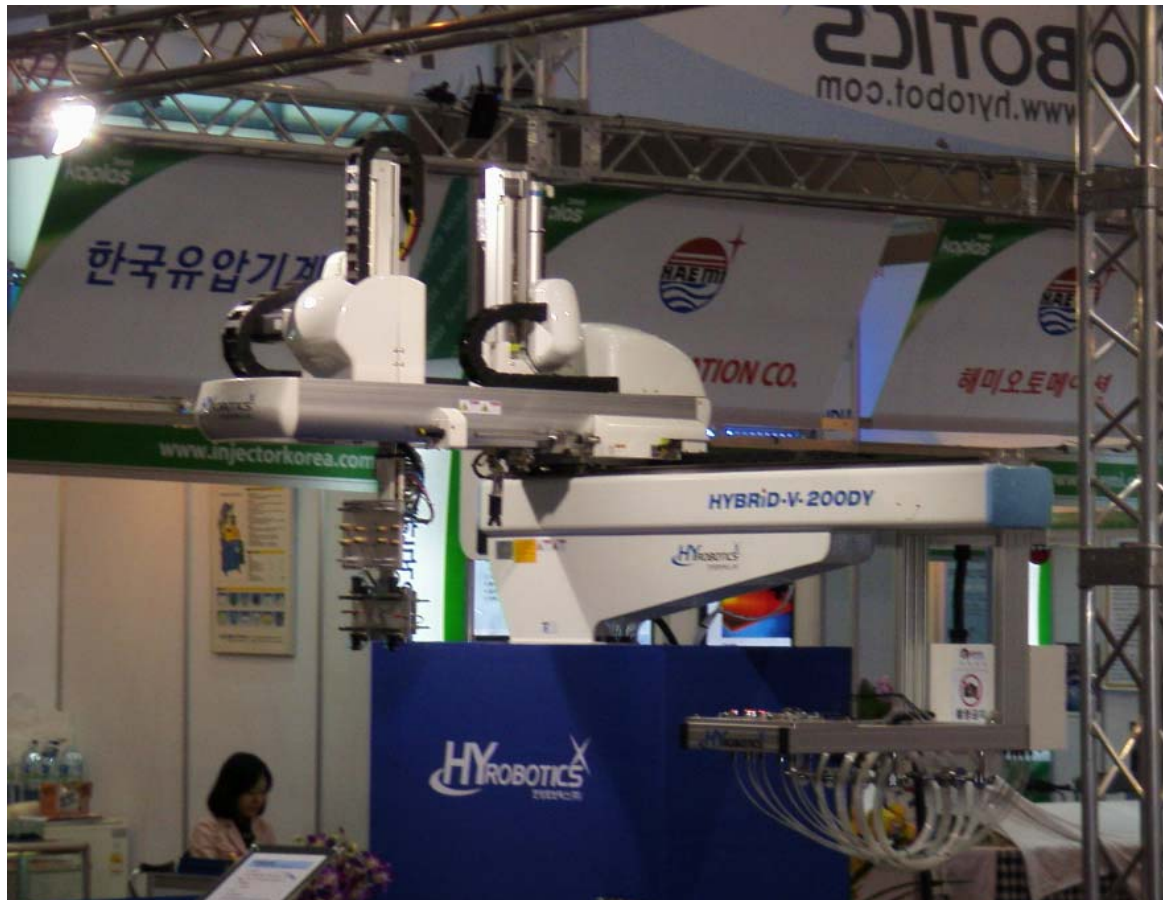
HYBRID SERIES ROBOT IN HYROBOTICS BOOTH : INSERT MOLDING AUTOMATION.
