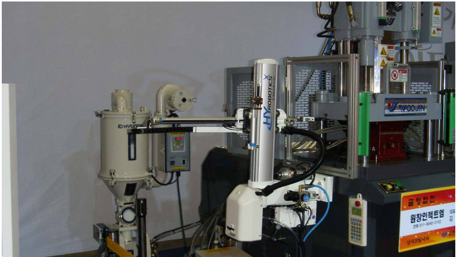
TOPIV SERIES ROBOT ON WOOJIN MOLDING MACHINES ( WOOJIN BOOTH ) VERTICAL 150 TONS
